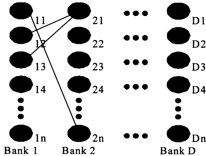
Figure 51: Flight Dependencies
