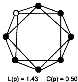
Figure 14: Regular Network
