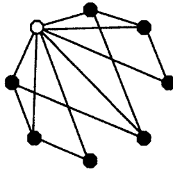
Figure 16: Hierarchical Network
