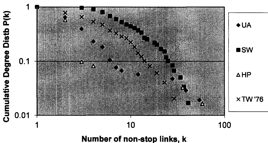
Figure 29: Different Airline Routing Strategies and Their Degree Distributions
